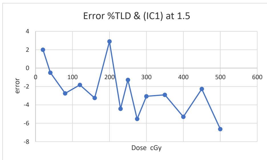
Figure. 1. Comparison of TLD and ion chamber C1 at the depth of 1.5 cm.
