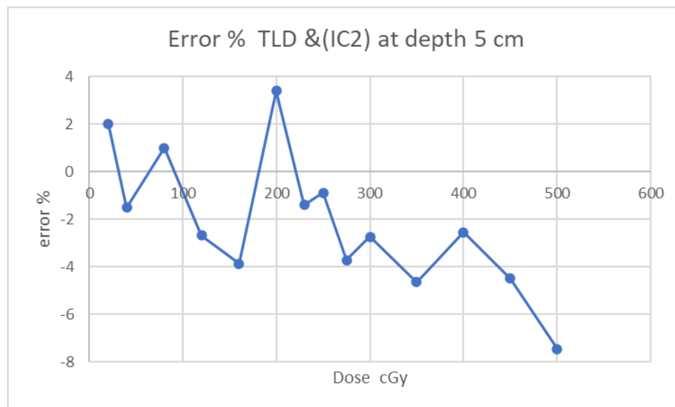
Figure. 4. Comparison of TLD and ion chamber C2 at the depth of 5 cm.
