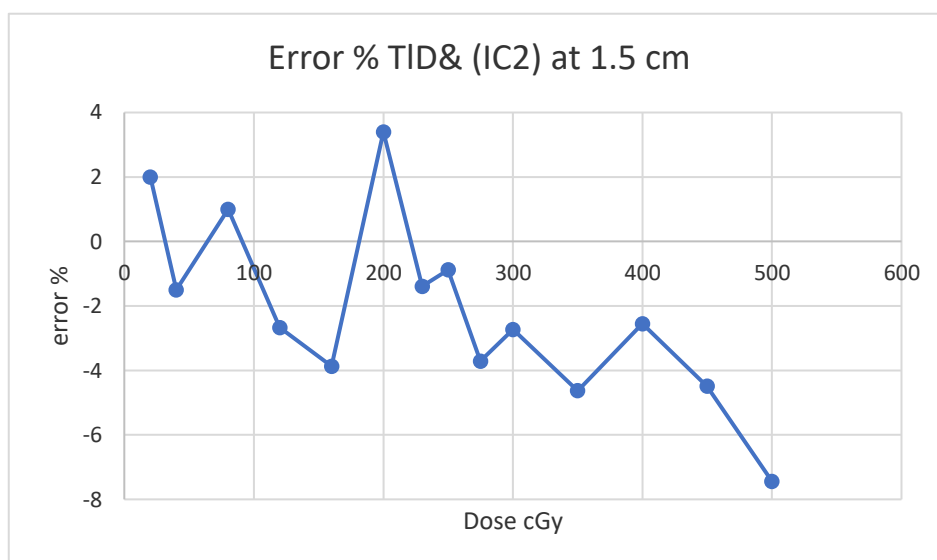
Figure. 2. Comparison of TLD and ion chamber C2 at the depth of 1.5 cm.
