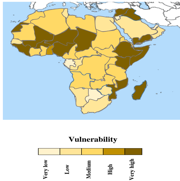
Fig (3): Map displaying susceptibility to hunger and climate change.
