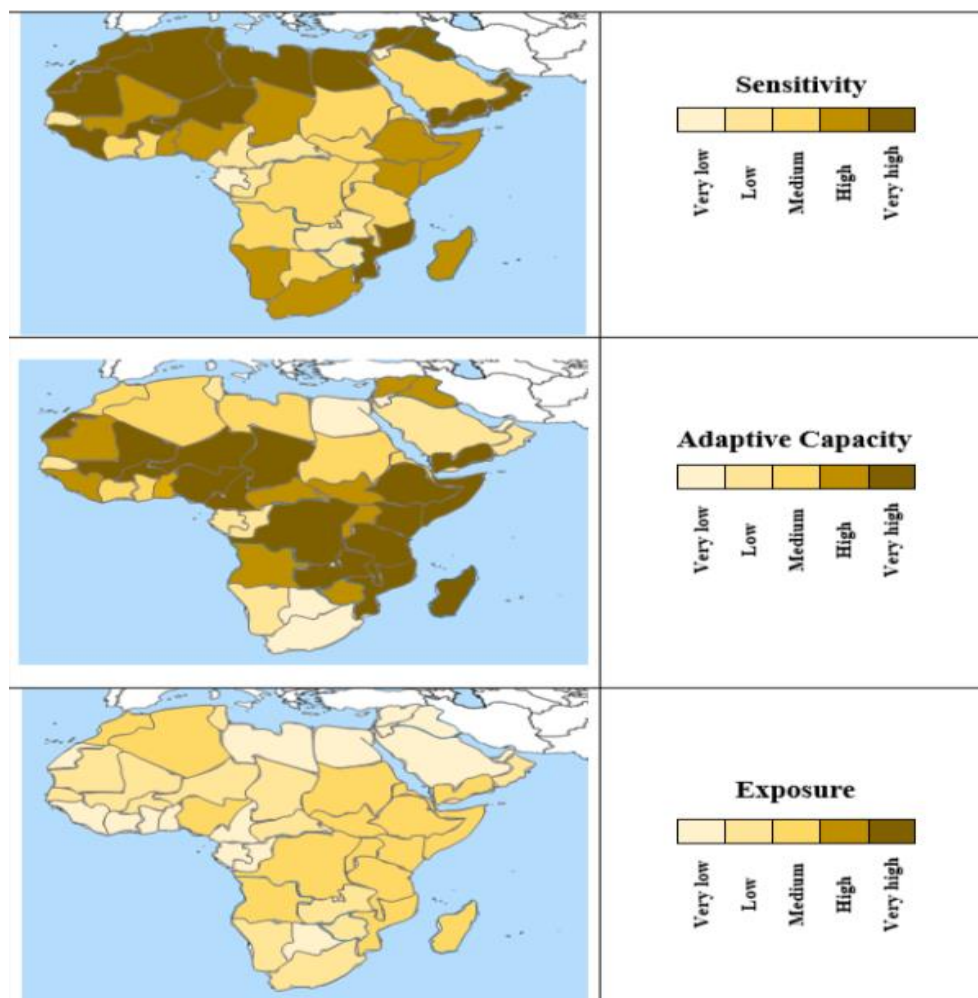
Fig (4): The distribution of the susceptibility components [16], including exposure (very low), adaptive capacity (low), and sensitivity (very high) for Egypt [current study].
