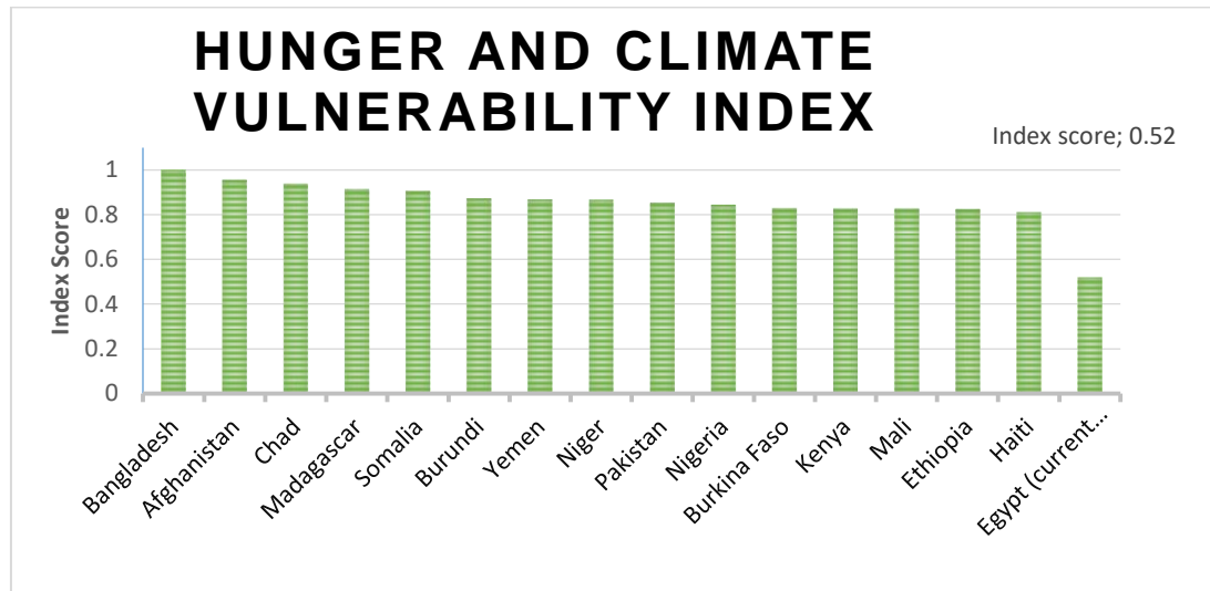
Fig (5): Climate Vulnerability Index.
