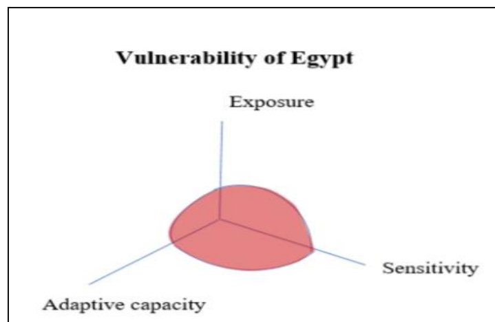
Fig (2): Vulnerability triangle for Egypt
