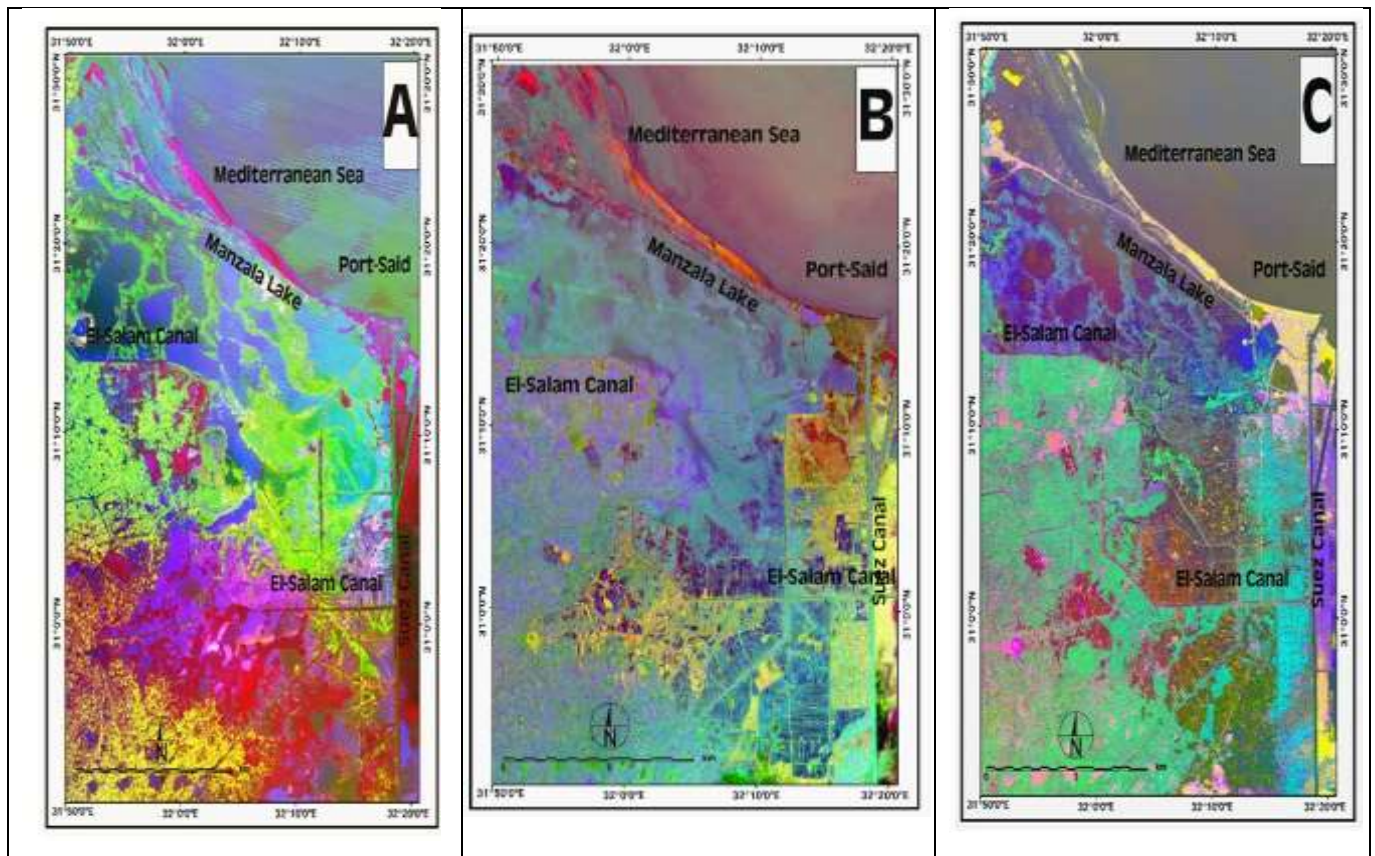
Figure 5. Enhanced PCA multi-temporal Landsat data of the PC1, PC2, and PC3 as RGB, showing the changes in the (LC-LU) classes in the NWSCR area where: A:1984 B:2000 C:2018.
